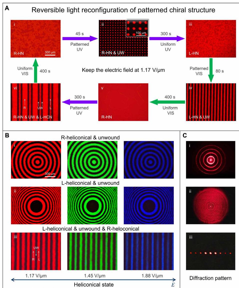
Fig. 4. Electric tunable micropatterns with prescribed microregions of molecular architectures by photopatterning. (A) Reversible photopatterning and photoerasing. (i) The PSS vis state of the uniform heliconical texture exhibiting homogeneous red reflection at an electric field of 1.17 V/μm. (ii) Dosage-controlled UV irradiation (1.8 mW/cm 2 ) through a photomask results in a two-dimensional (2D) circular pattern composed of periodic distribution of nematic and right-handedness heliconical regions. The inset shows the local enlarged micrograph of the 2D pattern. In exposed regions, the twist torque is reduced as a result of the decrease in the effective chirality, leading to the homeotropic state under the electric field. One may refer to the phototuning dynamics in Fig. 2C. (iii) Uniform abundant UV irradiation erased the afore-recorded pattern into the homogeneous left-handedness heliconical superstructure showing red reflection. (iv) Dosage-controlled visible irradiation (5.5 mW/cm 2 ) through a photomask results in a stripe pattern composed of periodic distribution of nematic and left-handedness heliconical regions. (v) Uniform abundant visible irradiation erases the afore-recorded pattern and transforms it into the homogeneous right-handedness heliconical superstructure. (vi) Abundant UV irradiation through a photomask results in 1D line grating composed of periodic left- and right-handedness heliconical regions. Uniform abundant visible irradiation erases the afore-recorded pattern into the homogeneous right-handedness heliconical superstructure state. The electric field is maintained as 1.17 V/μm throughout the whole process. (B) Reflection textures at different applied electric fields for (i) the concentric circles composed of regions of the nematic phase and the right-handedness heliconical superstructure, (ii) the Fresnel lens composed of regions of the nematic phase and the left-handedness heliconical superstructure, and (iii) the 1D line grating composed of regions of the right-handedness heliconical superstructure, the left-handedness heliconical superstructure, and the boundary nematic phase. (C) Diffraction patterns for (i) the circular grating, (ii) the Fresnel lens, and (iii) the 1D line grating at an electric field of 1.17 V/μm measured with an He-Ne laser beam at 632.8 nm. HN, heliconical state; UW, unwound state.
