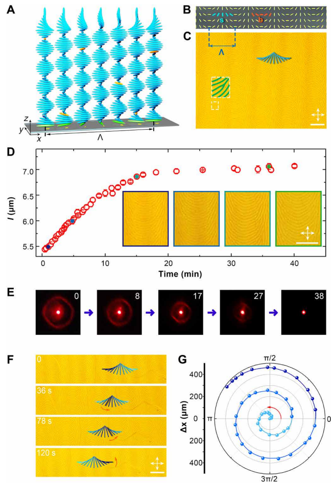
Fig. 2. Light-stimulated evolutions of photopatterned textures. (A) Helical configuration of the photopatterned CLC. (B) Schematic of the alignment condition. (C) POM texture of the generated periodic arch pattern. The group of blue bars denotes the local tangential directions of grating stripes in a single period. The inset illustrates a magnified texture with an edge dislocation. (D) Relationship between l and the exposure time. Insets are POM images of periodic arch patterns with different l during blue light exposure. The irradiance of blue light is about 100 \mu\text{W}/\text{cm}^2 . (E) Diffraction patterns during the exposure with exposure time labeled (min). (F) Light-stimulated shift of the periodic arch pattern. The exposure time is labeled in corresponding micrographs. (G) Dependency of \Delta x on \theta . White arrows denote the polarizer and analyzer transmission axes, respectively. Scale bars, 50 \mu\text{m} .
