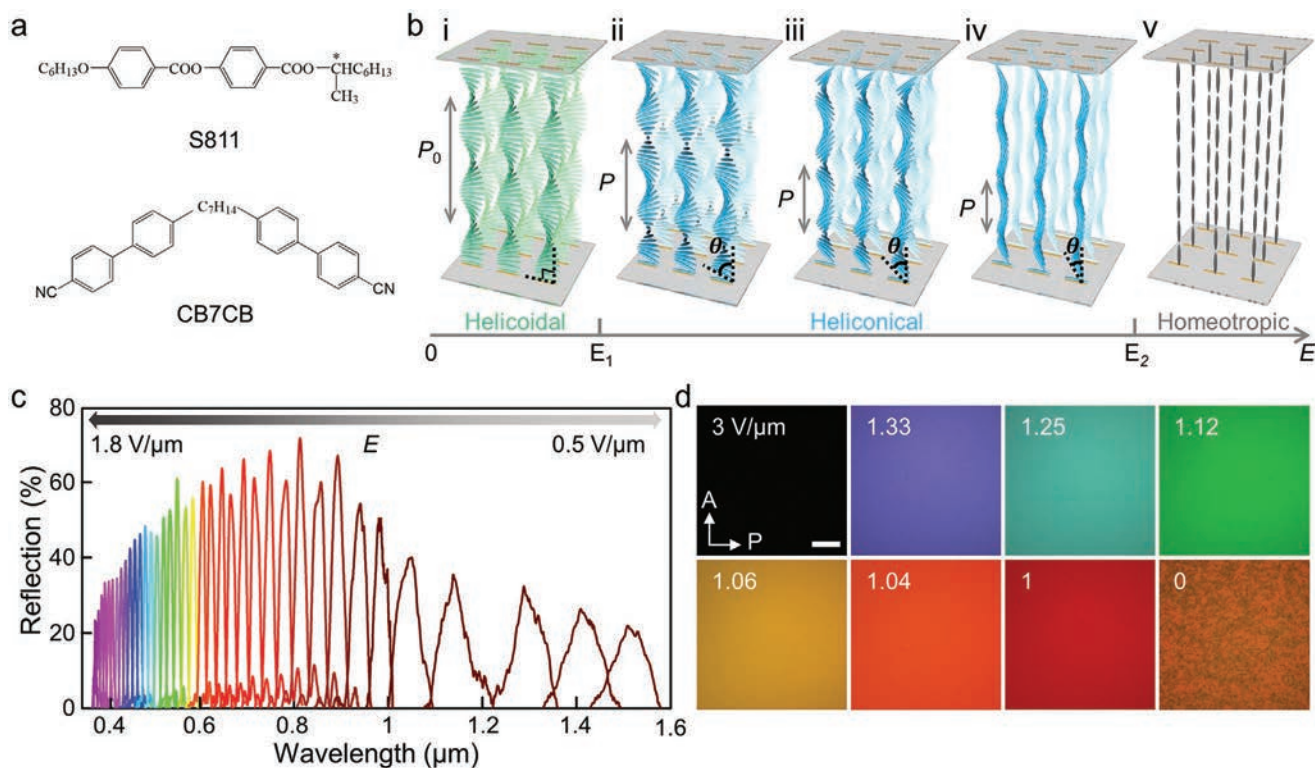
Figure 1. Helix transformation and performance of heliconical cholesterics under an electric field. a) Chemical structures of S811 and CB7CB. b) Schematic illustration of the helical superstructure under different external electric fields. i) Helicoidal superstructure with LC director perpendicular to the helical axis, E < E_1 ; ii–iv) Heliconical superstructures with LC director oblique to the helical axis, in which the oblique angle \theta gradually decreases as the electric field increases, E_1 < E < E_2 ; v) The unwound homeotropic nematic state with LC director parallel to electric field, E > E_2 . E_1 and E_2 are the thresholds of the transition from the helicoidal state to the heliconical state and the heliconical state to the homeotropic state. c) Bragg reflection spectra under incident circular-polarization light and d) POM textures of homogeneously aligned LC with different electric fields applied. The temperature of the cell is fixed at 26 °C. The scale bar indicates 200 μm for all micrographs.
