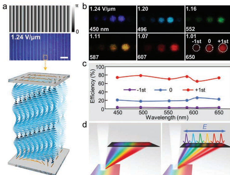
Figure 3. Experimental demonstration of broadband tuning by a fabricated helical PG. a) Theoretical director distribution, POM micrograph, and schematic illustration of PG. Black to white indicates the direction changing from 0^\circ to 180^\circ . b) Diffractive intensity distributions and c) wavelength-dependent diffraction efficiencies of PG. d) Schematic diagrams of the traditional grating and the proposed band-selective PG. The scale bar indicates 200 \mu\text{m} for all micrographs.
