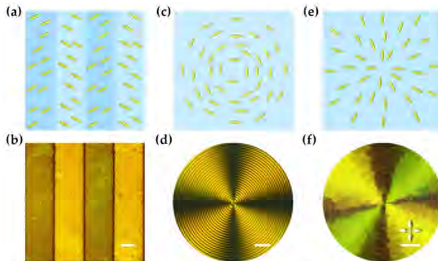
Figure 4. Photopatterned CLC gratings. (a,c,e) Schematic diagrams of binary, radial and angular alignments; (b,d,f) corresponding images of fingerprint textures. SD1 molecules are represented by yellow bars. White arrows denote the polarizer transmission axes. All scale bars indicate 50 \mu\text{m} .
