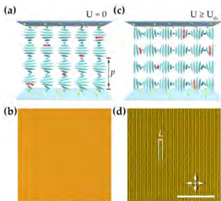
Figure 1. Homogeneously aligned photo-responsive cholesteric liquid crystals (CLCs). (a,c) Schematic diagrams and (b,d) corresponding POM images of the planar texture and the electric field-induced grating. The chiral dopants, SD1 and LC molecules are marked by red, yellow and light blue rods, respectively. White arrows denote the transmission axes of polarizer and analyzer. The scale bar is 50 \mu\text{m} .
