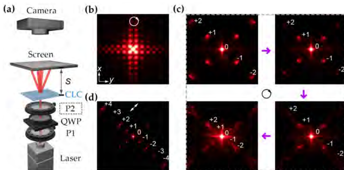
Figure 3. Diffraction performance of checkerboard hierarchical gratings. (a) Schematic diagram of the light path. P and QWP represent the polarizer and the quarter wave plate, respectively. P1 and QWP are utilized to produce circularly polarized light. P2 is used to generate linearly polarized light; (b) diffraction pattern from the checkerboard hierarchical gratings; (c) optical tuning of the diffraction orders at T = 0 min, 5 min, 10 min, and 20 min, respectively; (d) polarization-dependent diffraction pattern. Circular and white arrows denote the polarization state of incident light.
